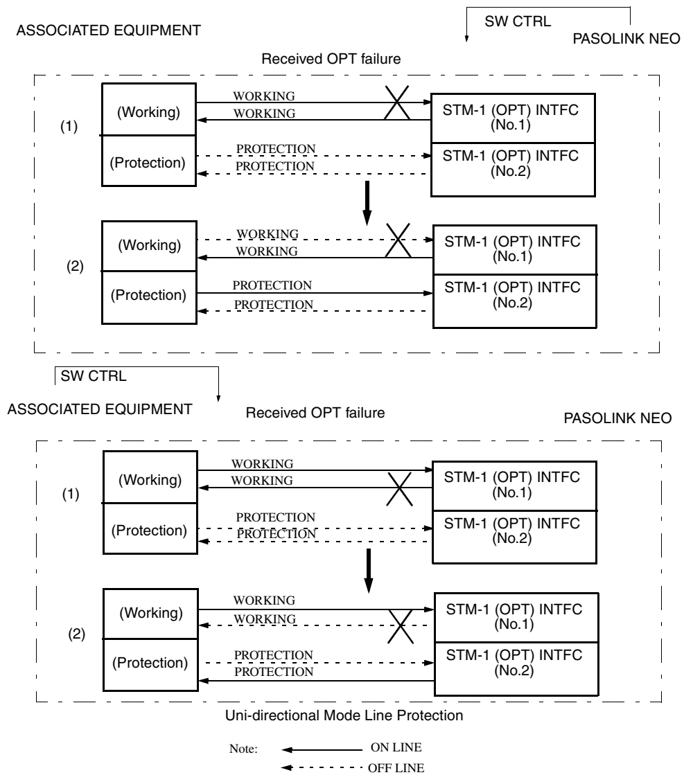
Fig. 3-3 Line Protection
