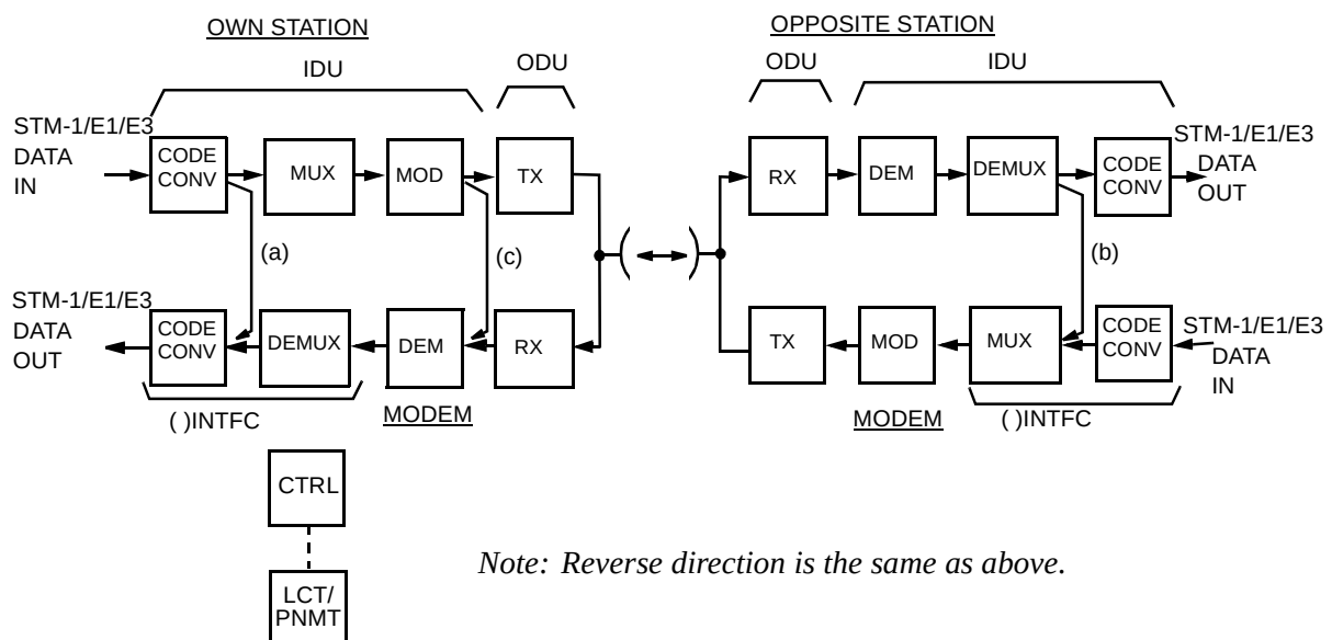
Fig. 3-5 Loopback Location
